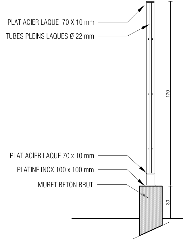
DETAIL CLOTURE ACIER Ech:1/20ème
