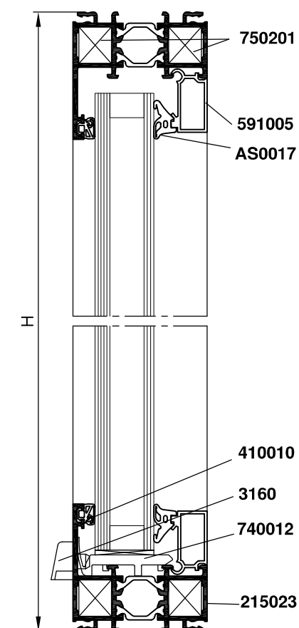
Variante dormant rainure parclose drainage apparent
