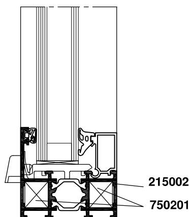
Variante dormant rainure parclose drainage apparent
